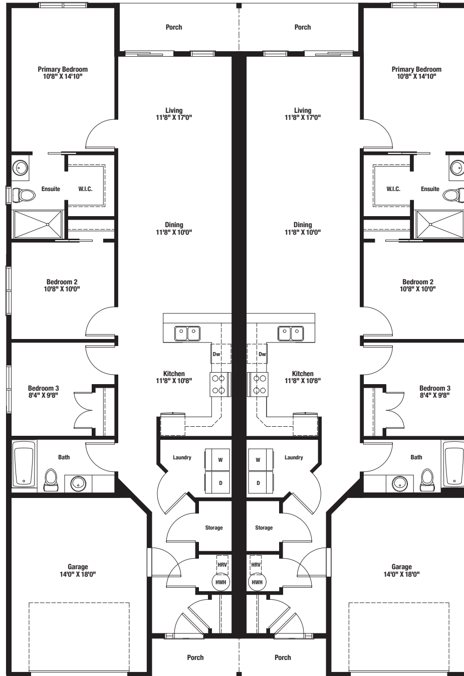
First Floor
